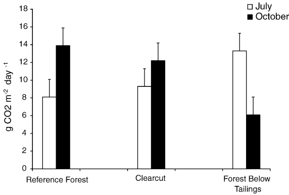
Fig. 3. Average respiration rates for forest soils in July and October 1999. The reference forest soil was adjacent and 100 m north of the Alder Mine and the clear-cut was at the same altitude on the opposing slope of the Alder Creek valley. Error bars indicate S.D.
