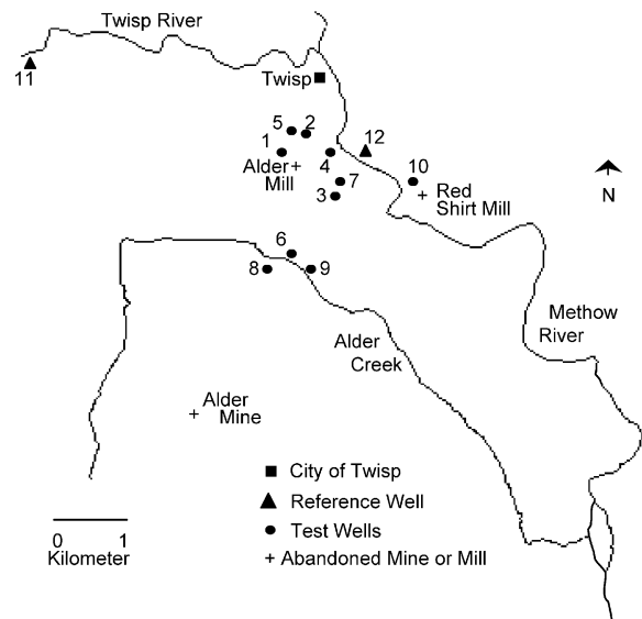
Fig. 2. Location of private drinking water wells and locations where groundwater samples were collected in the vicinity of the contaminant sources at Alder Mine, Alder Mill and Red Shirt Mill. Reference wells number 11 and 12 are also identified.
