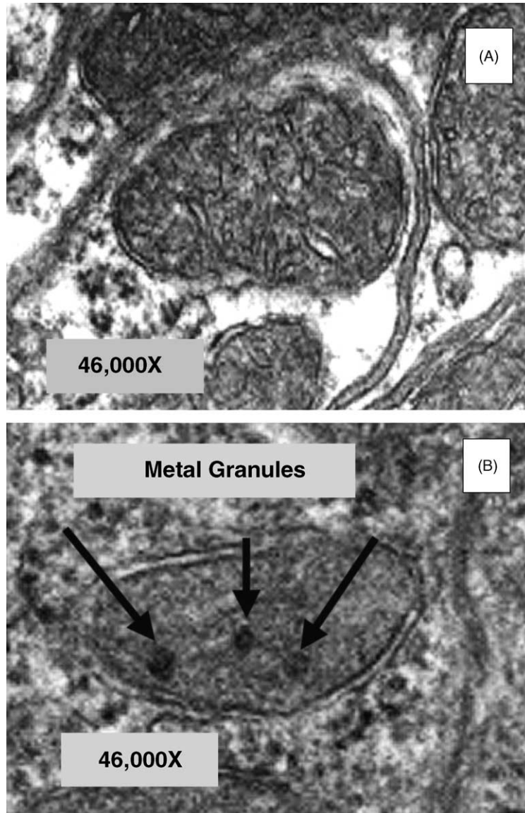
Fig. 7. TEM micrographs of mitochondria in hepatocytes from juvenile triploid trout ( O. mykiss ) fixed in Karnovsky's (5% glutaraldehyde and 4% formaldehyde in 0.1 M cacodylate buffer), embedded in Eponate, and contrasted with uranyl acetate and lead citrate. Duplicate samples not contrasted with uranyl acetate and lead citrate were also prepared to control for the effects of staining on the presence of electron-dense granules in mitochondria. (A) Stained section from trout maintained 7 weeks in pens upstream from the abandoned mine sites (station 13) and (B) stained section from trout maintained 7 weeks in pens downstream from the abandoned mine sites (station 17).
