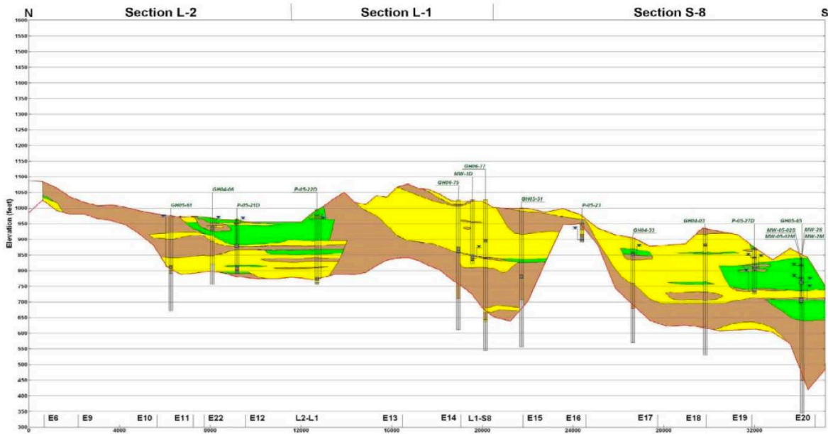
Figure 2. Hydrogeologic cross section from the Pebble prospect mine lease illustrates complexity of subsurface sediment layers, which influence groundwater flow paths. Colors represent different sediment layers with: brown = sand or silty sand; green = clay or silty clay, and yellow = gravel and gravelly sand. Graphic from Smith and McCreadie (2008).
